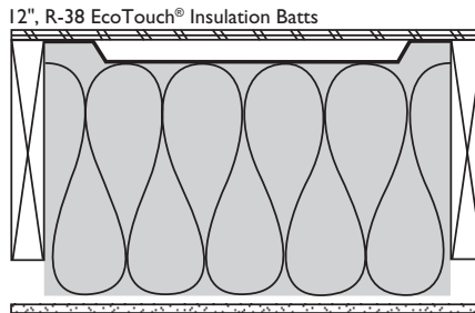
Standard Batt's compressed into a 11¼" cavity with ventilation baffle added to allow 1" air space deliver approximately R-35.
