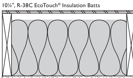
New R-38C batts provide the recommended ventilation air space when properly installed and deliver a full R-38.
