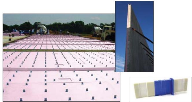
Thermomass System SC, tilt-up with FOAMULAR® 250
