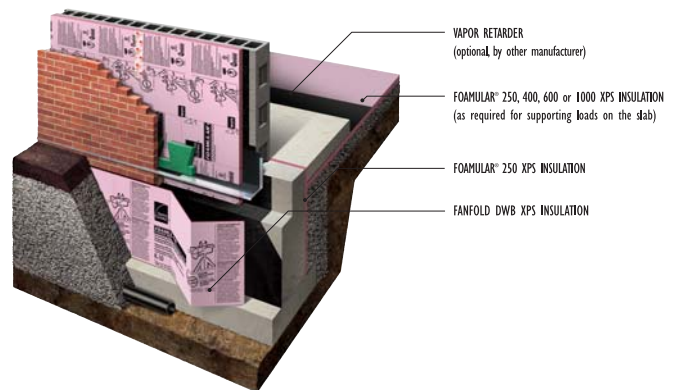
Foundation Insulation, Waterproofing Protection, Slab Edge Insulation
