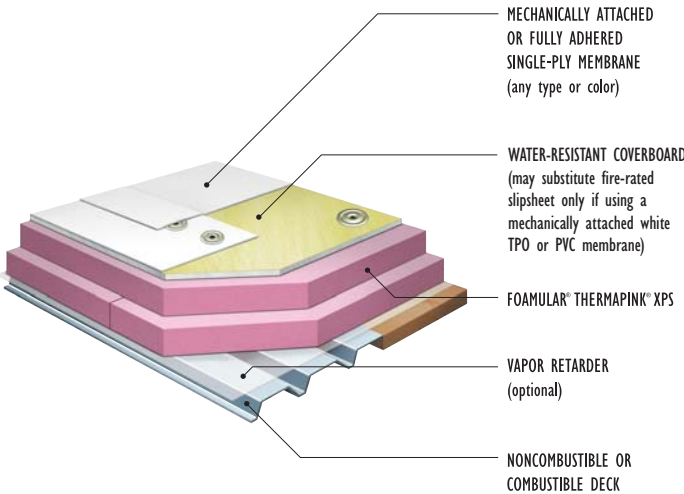
System with Cover Board
